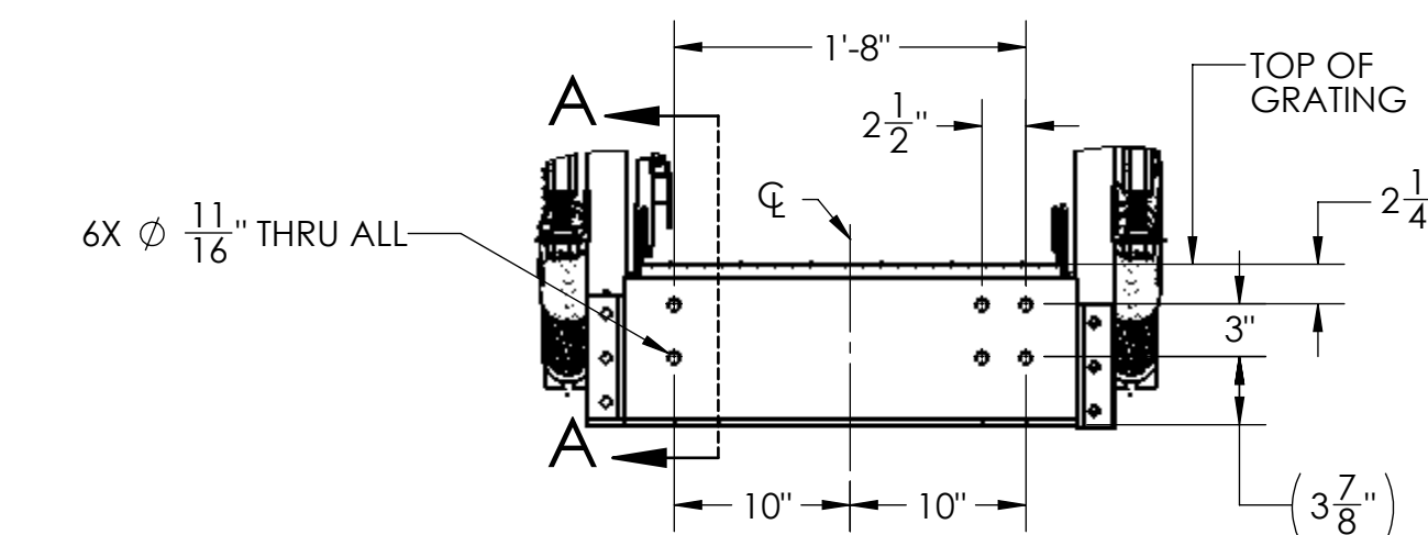
MOUNTING BOLT PATTERN
