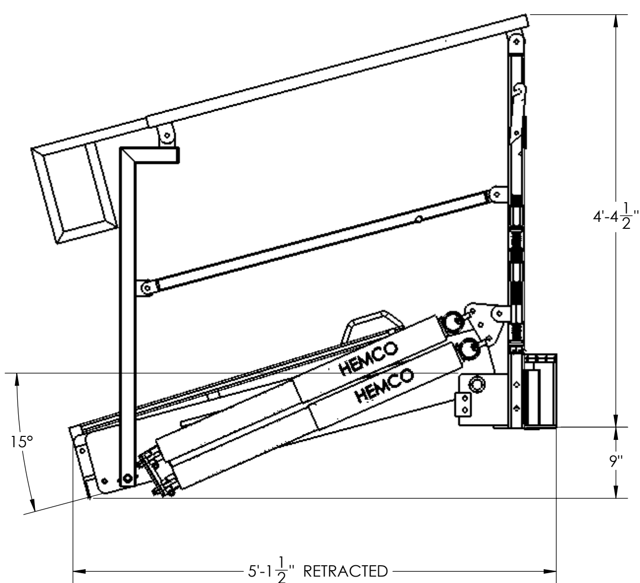
15° DECLINE EXTENSION IN
