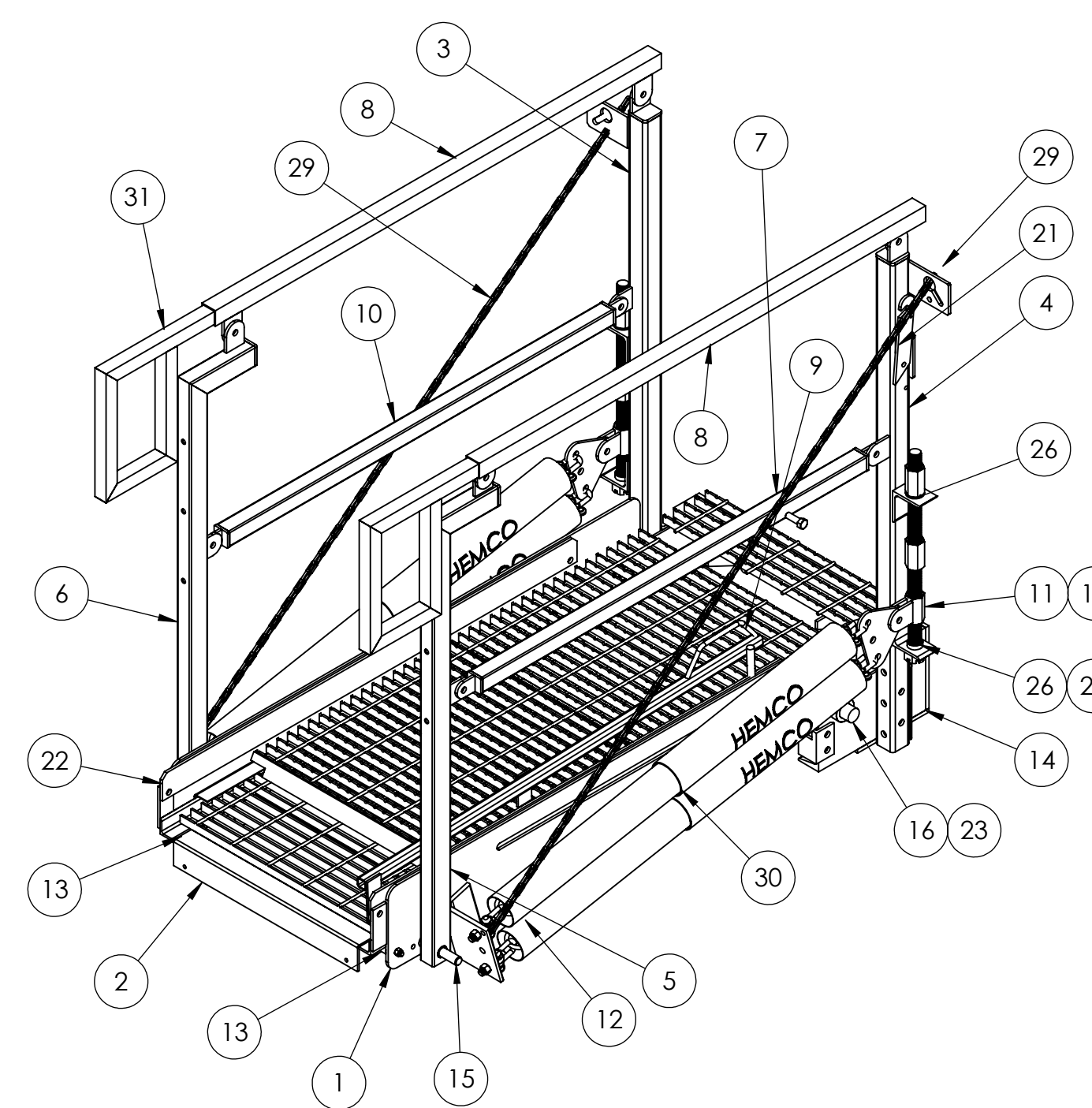
ISO VIEW
