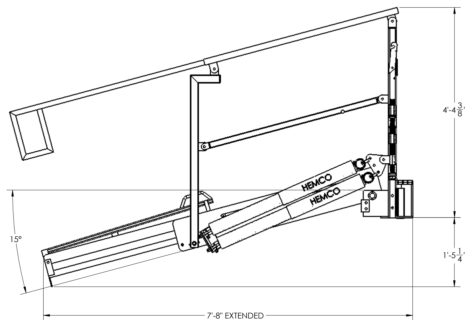
15° DECLINE EXTENSION OUTWARD
