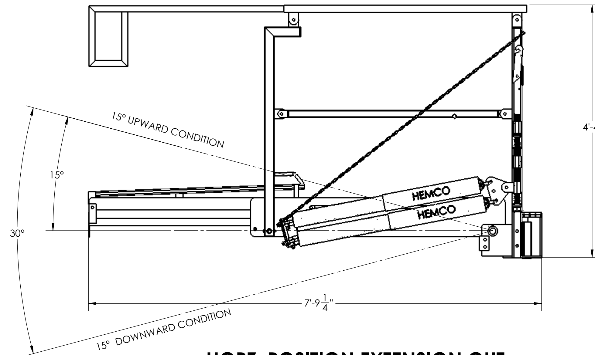
HORZ. POSITION EXTENSION OUT
