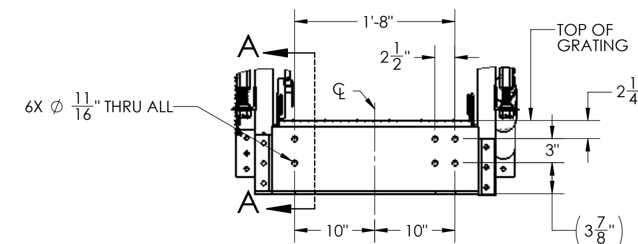
MOUNTING BOLT PATTERN
