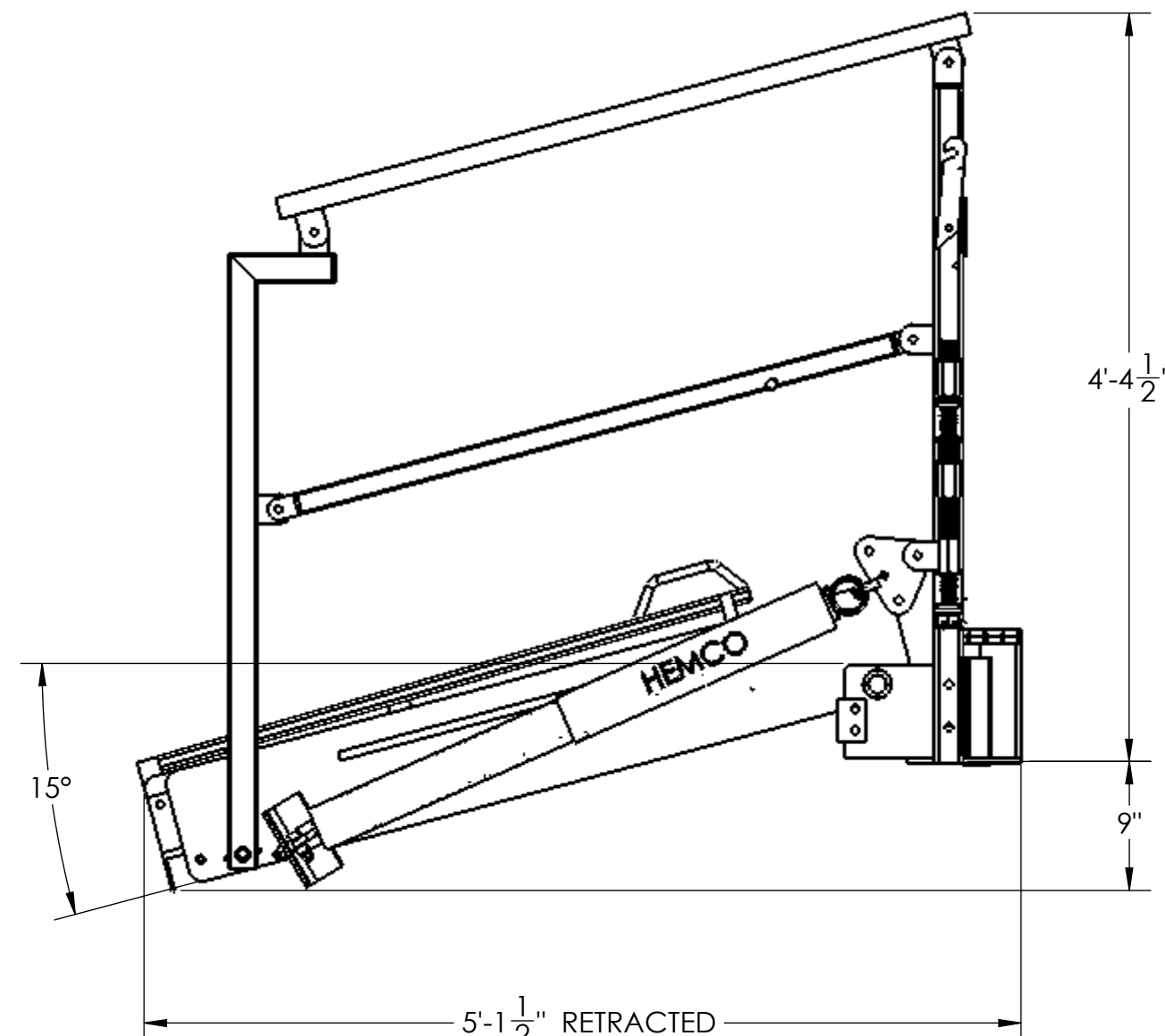
15° DECLINE EXTENSION IN
