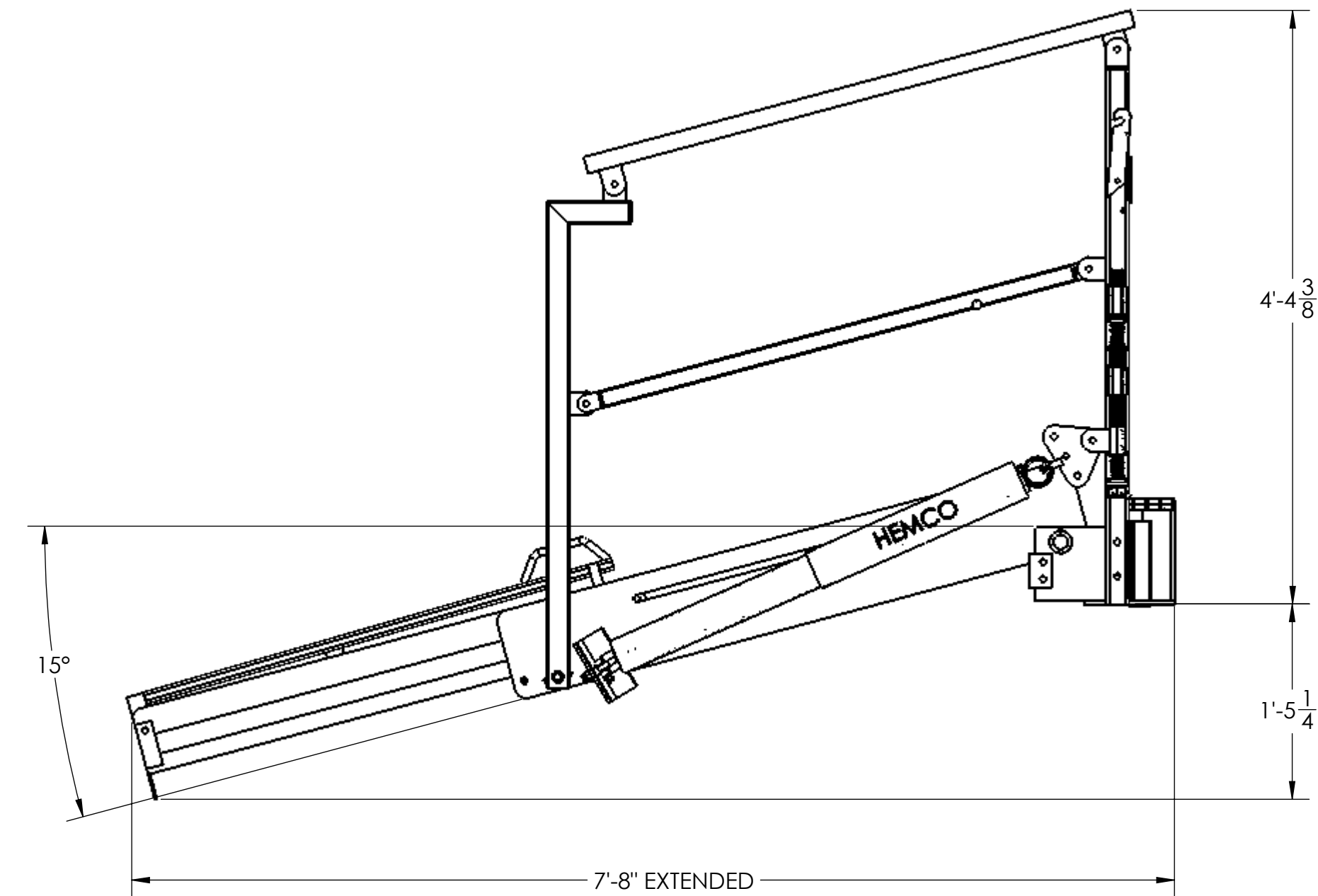
15° DECLINE EXTENSION OUTWARD
